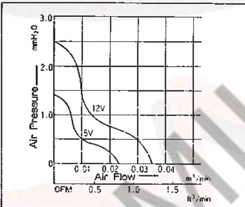
AIR FLOW VS AIR PRESSURE
