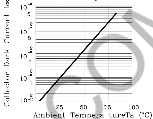
Fig. 2 Collector Dark Current vs. Ambient Temperature
