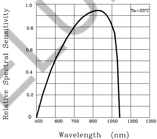
Fig. 5 Spectral Sensitivity
